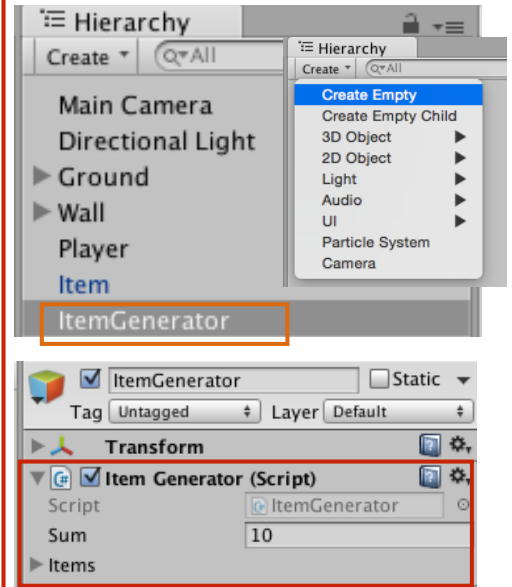
ItemGenerator.cs
